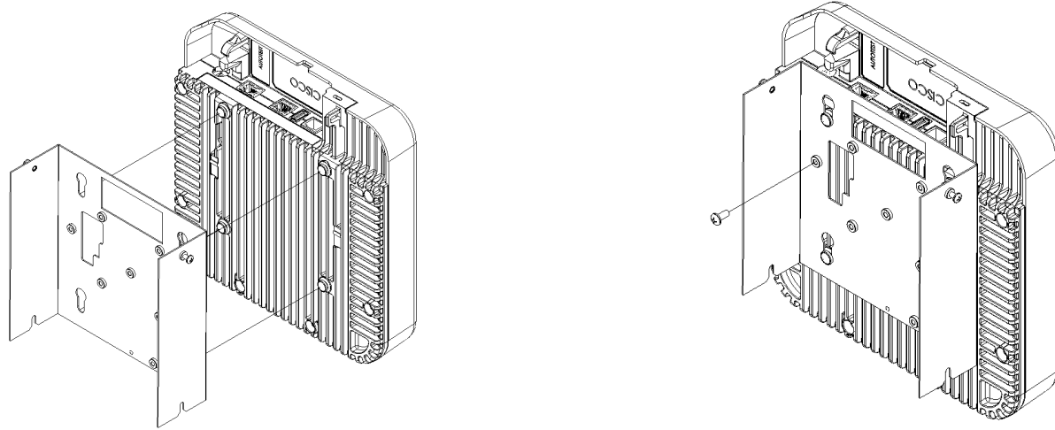
Figure 5 - Cisco 2800, 3800 Installation
