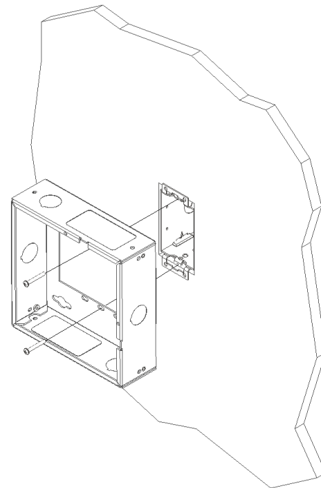
Figure 1 - Surface Mount Over Outlet
