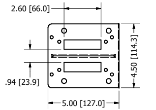
Right Angle Bracket
