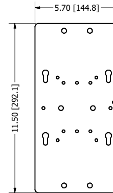
Cisco Mounting Bracket
