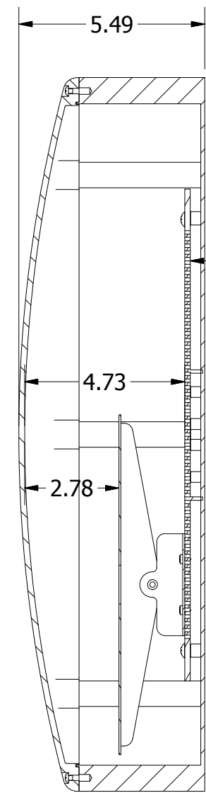
SECTION A-A SCALE 1 / 4
